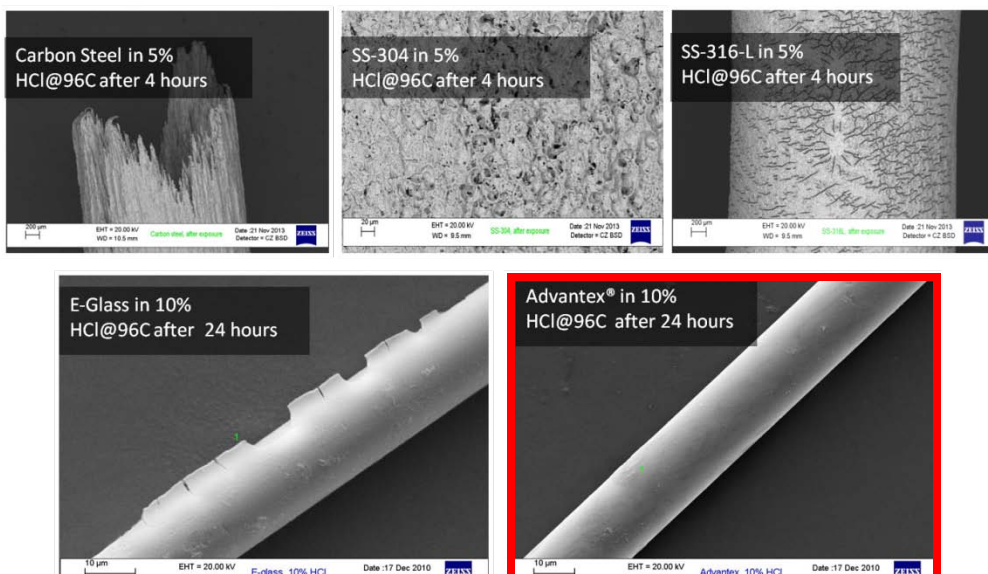
Figure 2 Performance of CS, SS-304, SS-316-L, E-Glass, and Advantex® glass after exposure to hydrochloric acid
